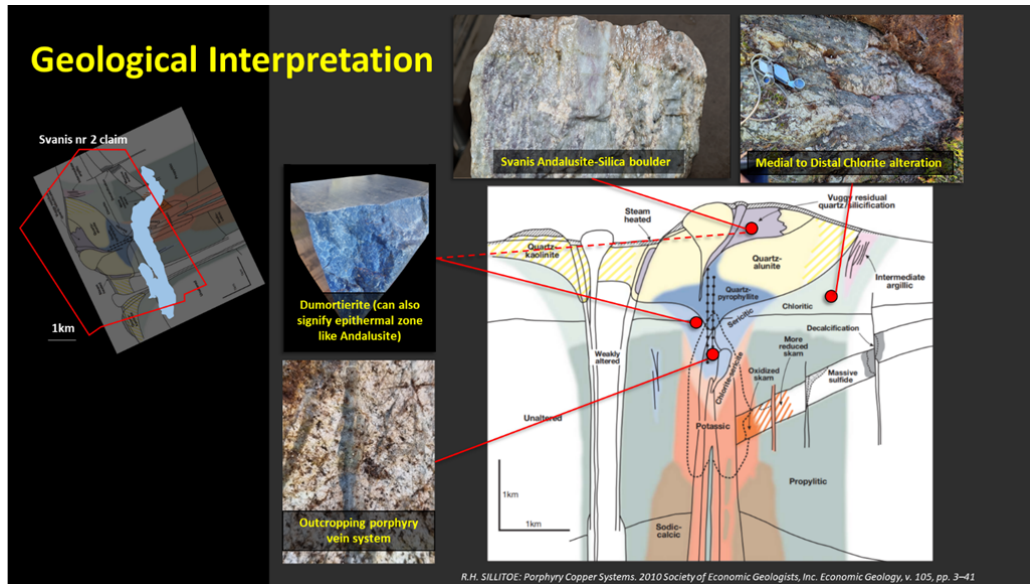
Figure 6: Swan Lake Project - Geological Interpretation
