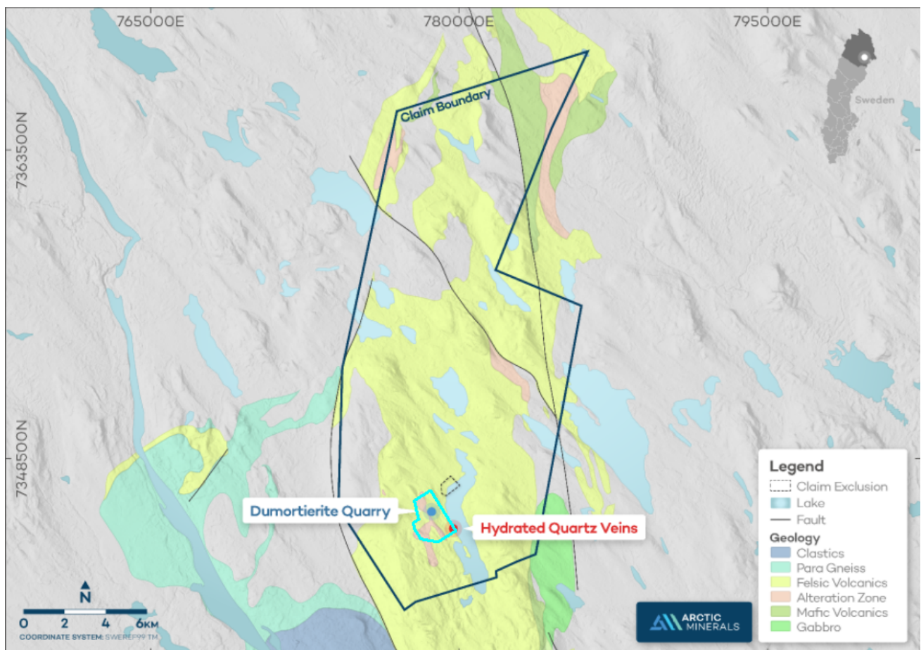
Figure 4: Swan Lake Project - Local Geology. Gra-IP survey in cyan
