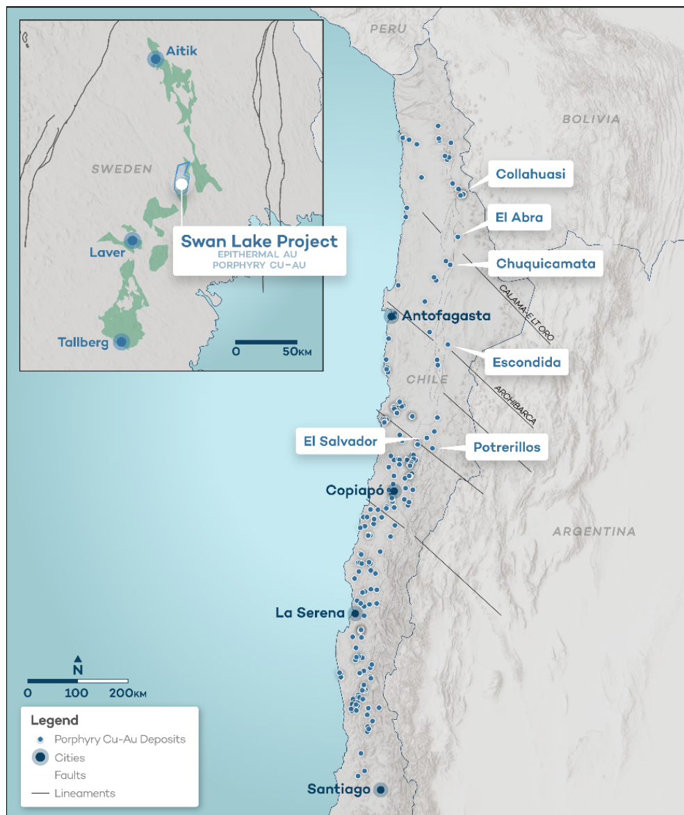
Figure 3: Northern Sweden's Porphyry District in comparison with classical Chile porphyry region
